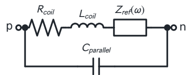
(c) Reduced ICP coil one-port
