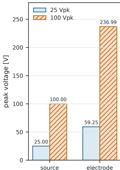
(a) Voltage amplitude
