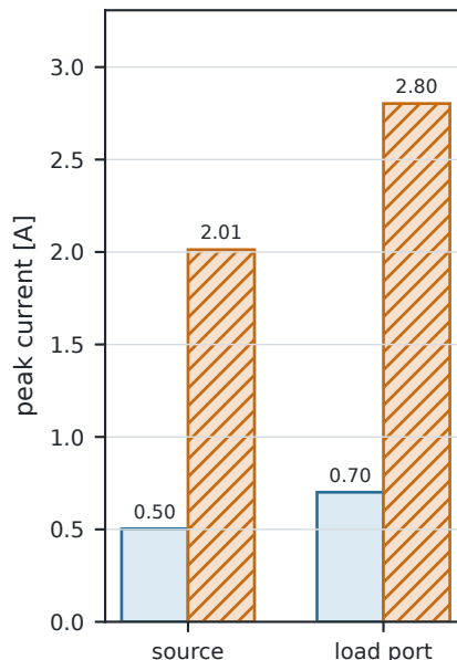
(b) Current amplitude
