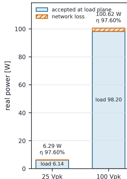
(c) Power disposition
