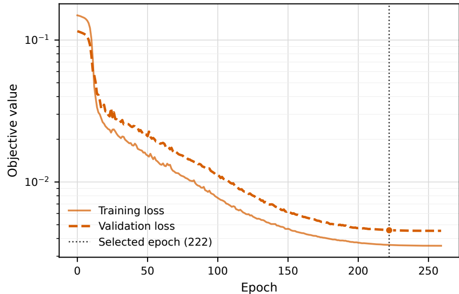
DeepONet (POD)
