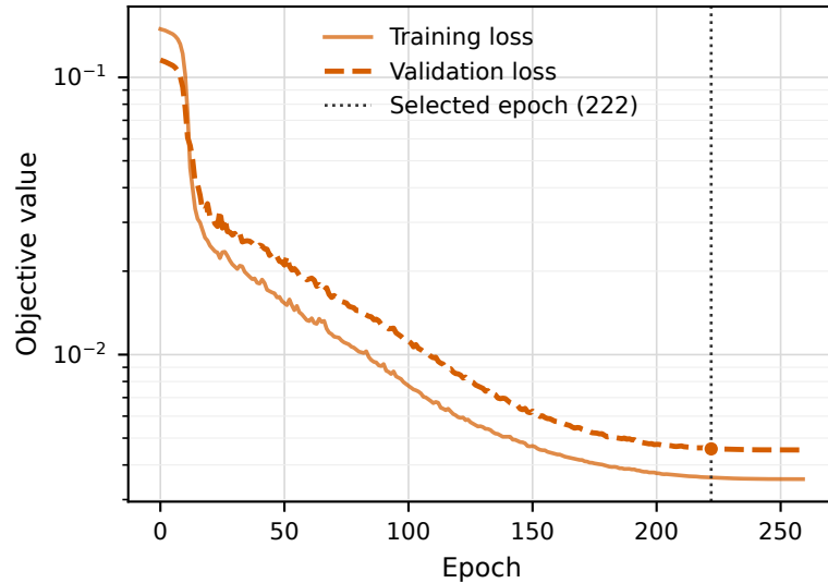
DeepONet (POD)
