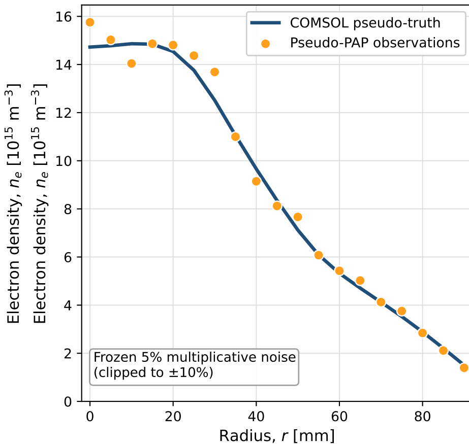
Measured radial distribution at z = 12.7 mm
