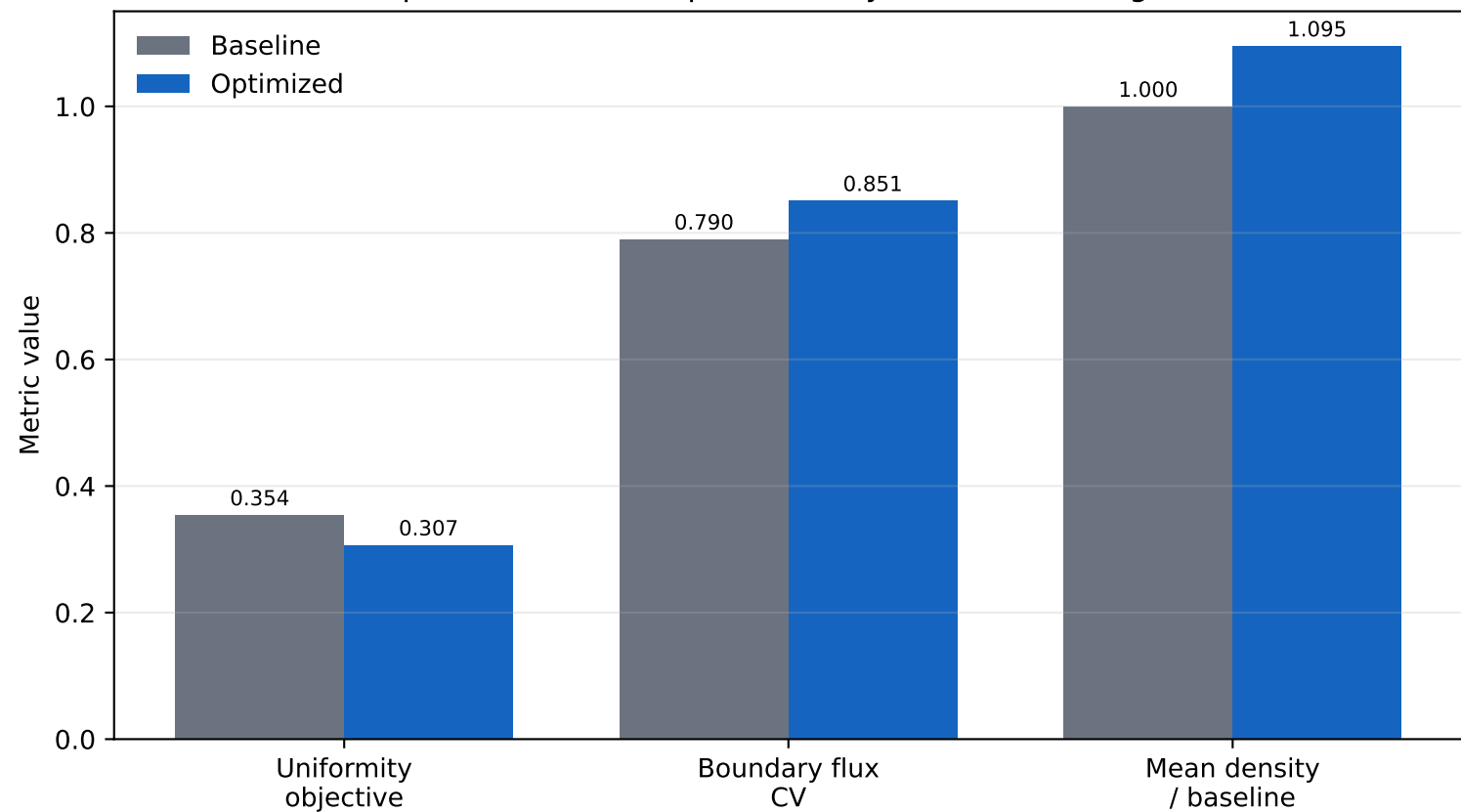
Optimization effect predicted by the FFNO surrogate
