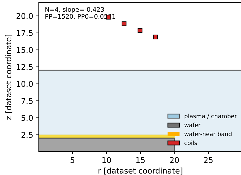
Chamber, wafer and coil layout
