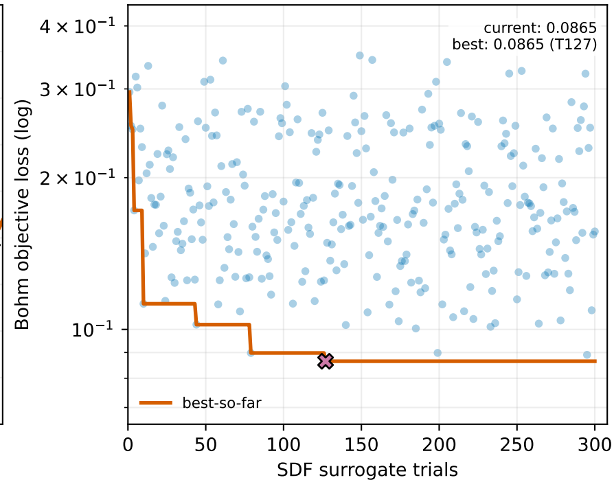
Joint search: 2-5 coils
