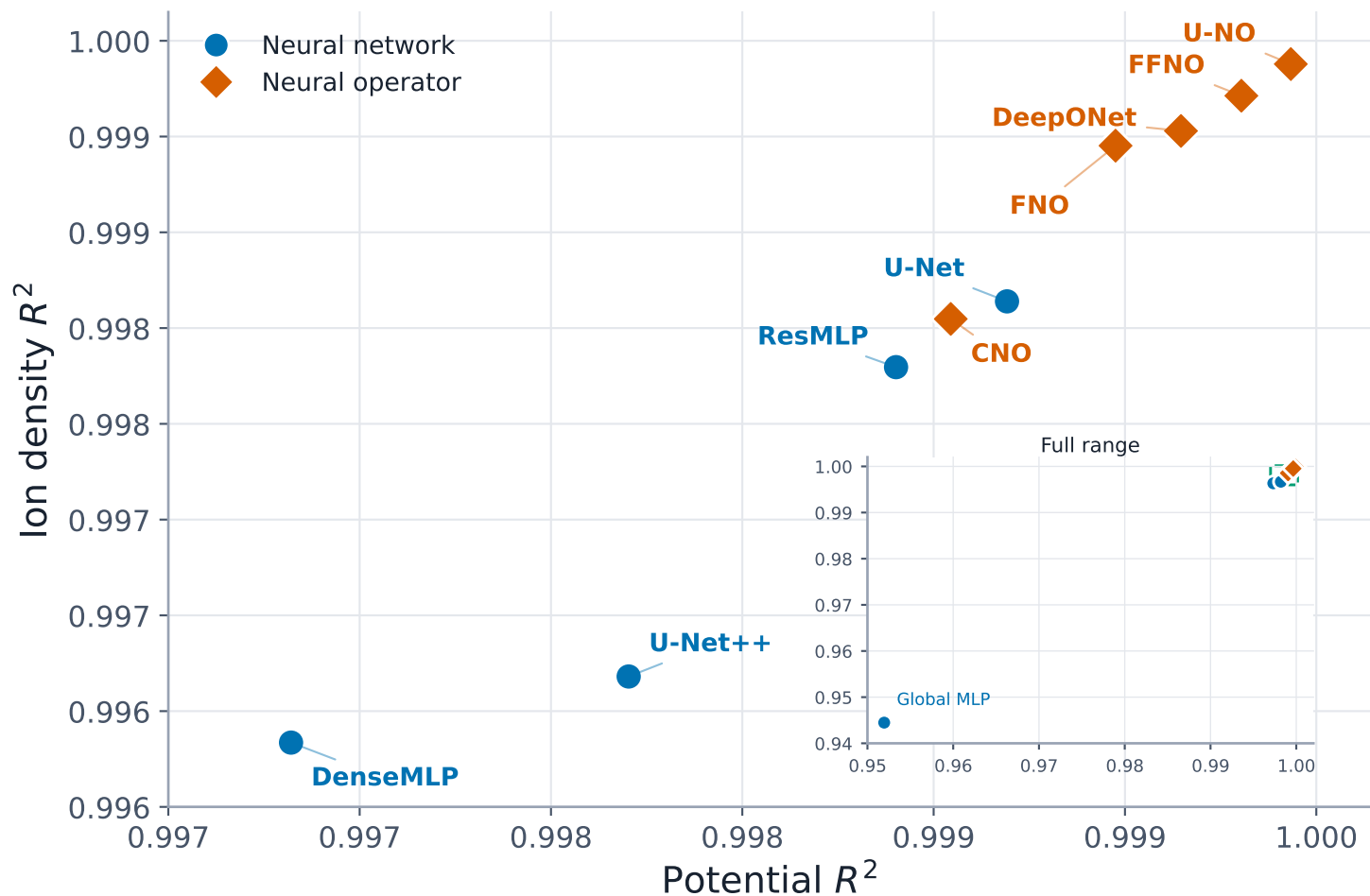
Ion density vs. potential: test R^2
