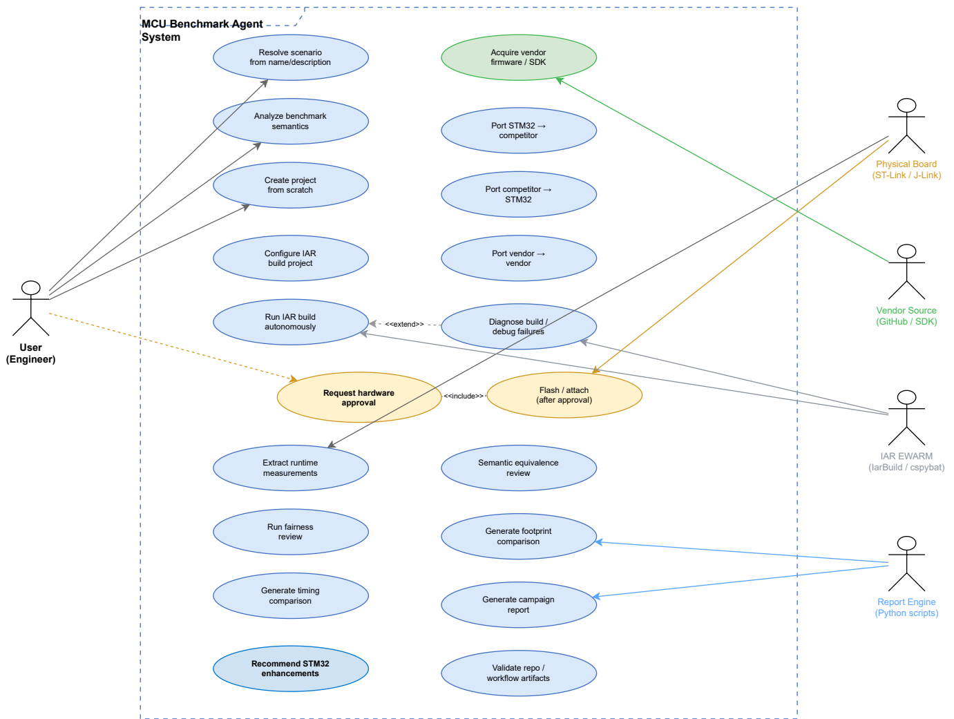
Figure 5.2: UML use case diagram of the MCU Benchmark Copilot Agent system. Blue ellipses represent autonomous use cases; yellow ellipses require user approval; green indicates external acquisition. External actors include the user, physical board, vendor source repositories, IAR EWARM toolchain, and the report engine scripts.
