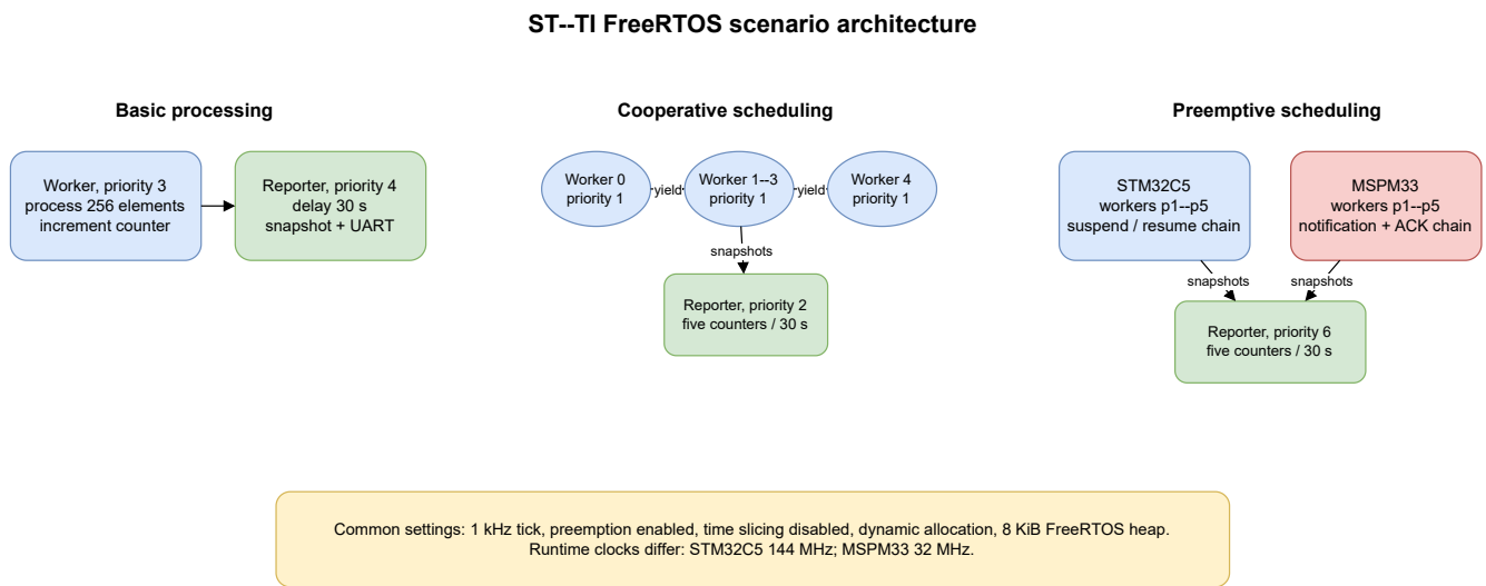
Figure 7.4: Task architecture of the three ST–TI FreeRTOS scenarios. The preemptive scenario deliberately shows the non-equivalent synchronisation paths found in the measured projects.
