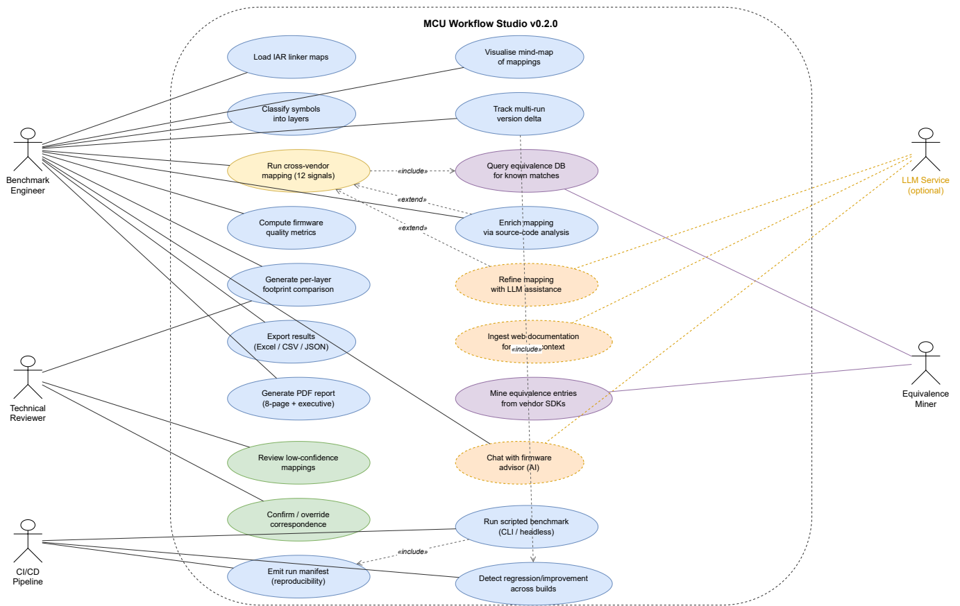
Figure 4.2: UML use-case diagram of MCU Workflow Studio v0.2.0. Five actors interact with twenty use cases grouped by concern: the benchmark engineer drives the core analysis, the technical reviewer validates low-confidence mappings, the CI/CD pipeline runs scripted headless benchmarks, the LLM service (optional, dashed) enriches the mapping, and the equivalence miner maintains the cross-vendor knowledge base.
