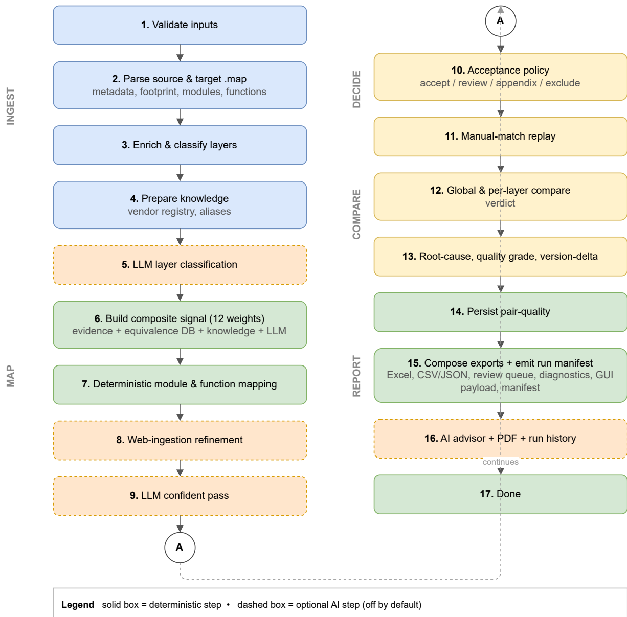
Figure 4.5: End-to-end benchmark pipeline, from linker-map ingestion to report generation. Dashed stages are optional AI-assisted steps that are disabled by default; the solid deterministic path runs end to end on its own.
