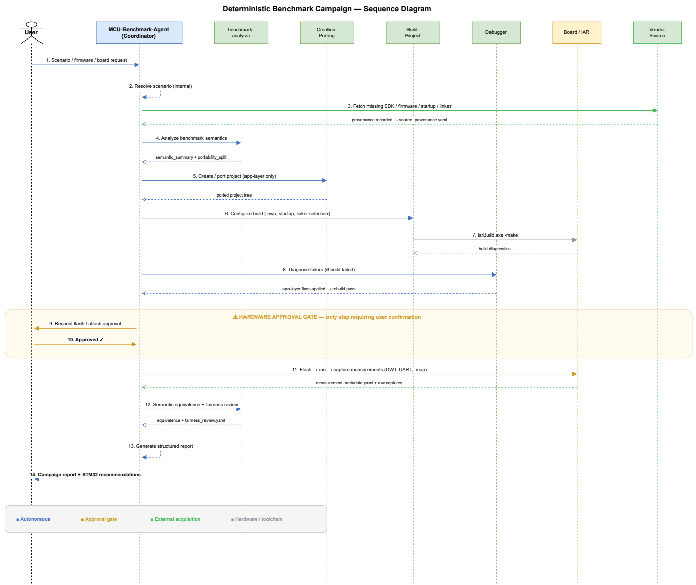
Figure 5.6: UML sequence diagram of a deterministic benchmark campaign. The coordinator delegates to specialist agents (benchmark-analysis, Creation-Porting, Build-Project, Debugger) and interacts with external actors (Vendor Source, Board/IAR). The hardware approval gate (steps 9–10, highlighted) is the only point requiring user confirmation; all other steps execute autonomously.
