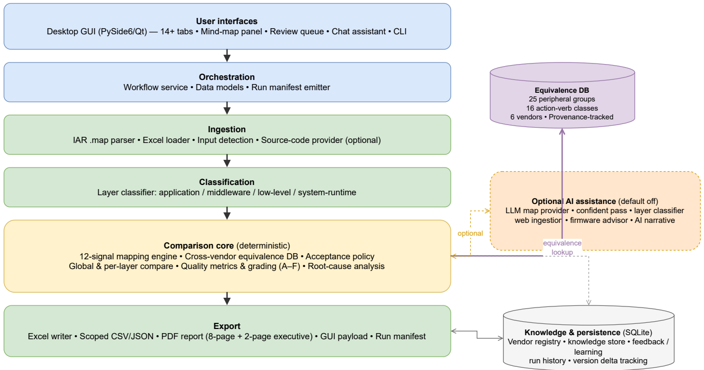
Figure 4.1: Layered architecture of the footprint-analysis tool. A deterministic comparison core (ingestion, classification, mapping, comparison, export) is wrapped by the user interfaces and backed by an SQLite knowledge base; an optional, off-by-default AI-assistance column refines the mapping without ever sitting on the critical path.
