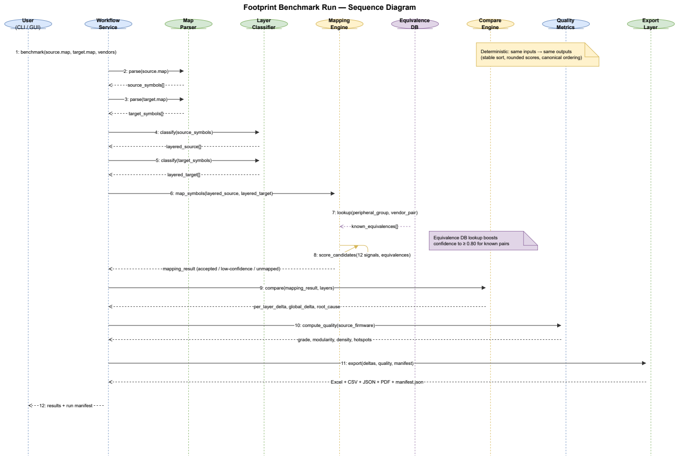
Figure 4.3: UML sequence diagram of a complete footprint benchmark run. The workflow service orchestrates twelve steps: parsing both linker maps, classifying symbols into layers, querying the equivalence database, scoring candidates with twelve weighted signals, computing per-layer deltas, evaluating firmware quality metrics, and emitting the run manifest alongside all export artefacts.
