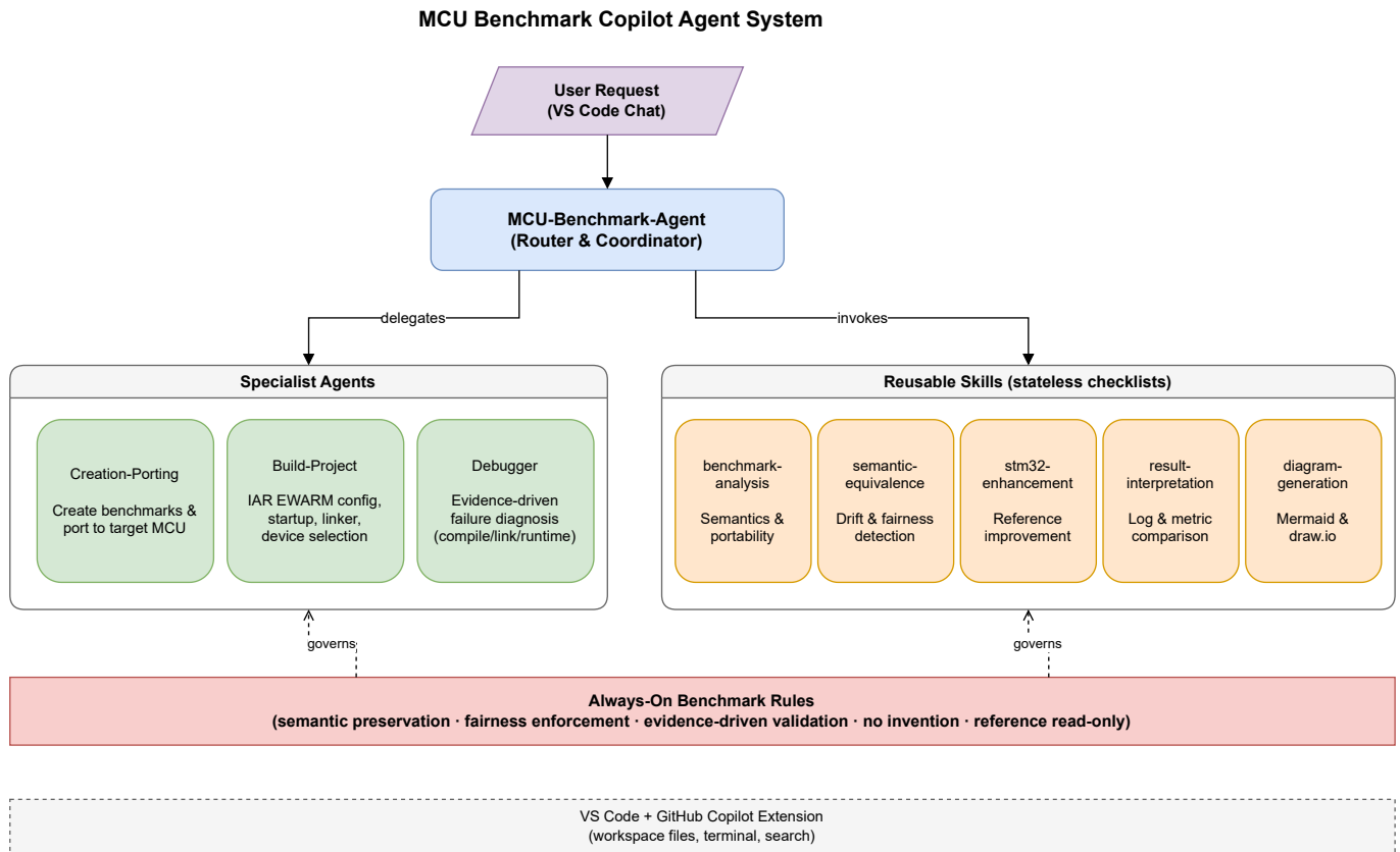
Figure 5.1: Architecture of the MCU Benchmark Copilot Agent system. The coordinator resolves scenarios and delegates to specialist agents; automation tools handle deterministic build/measurement operations; all layers operate under the shared always-on benchmark rules and consult the configuration registry.
