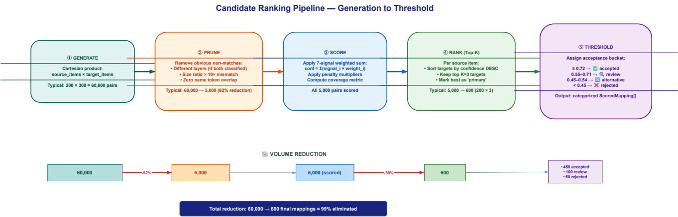
Figure 2.9: Candidate generation, ranking, and threshold flow. The Cartesian product of source and target items is pruned by fast rejection filters, scored on all signals, and bucketed into accepted, review, alternative, and unmatched categories by confidence thresholds.
