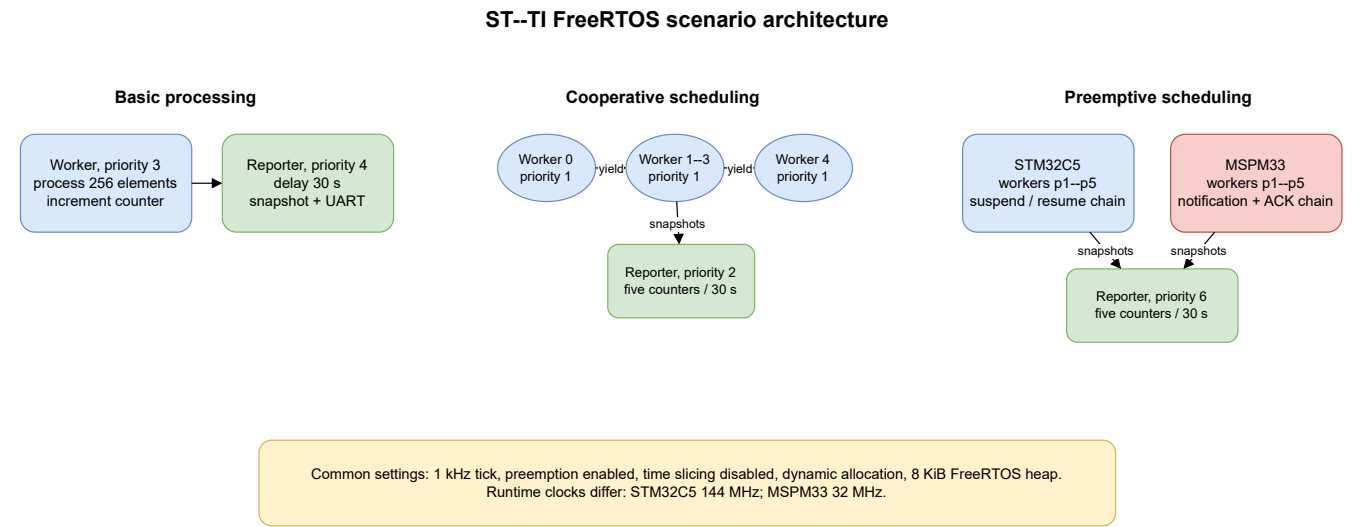
Figure 5.4: Task architecture of the three ST--TI FreeRTOS scenarios. The preemptive scenario deliberately shows the non-equivalent synchronisation paths found in the measured projects.
