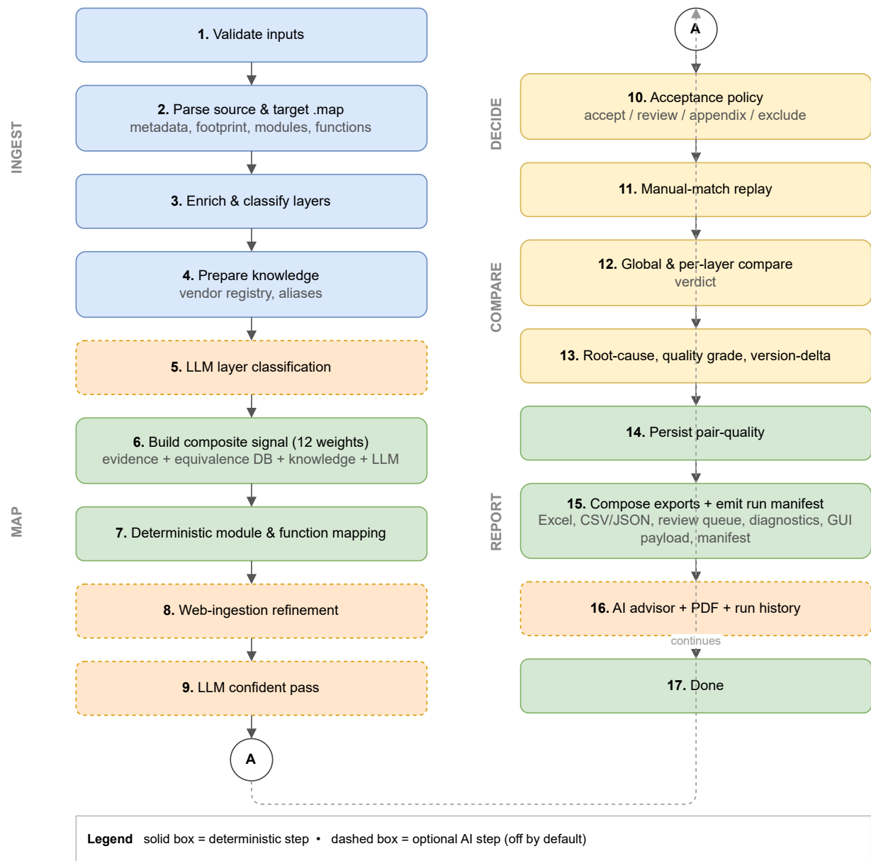
Figure 2.5: End-to-end benchmark pipeline, from linker-map ingestion to report generation. Dashed stages are optional AI-assisted steps that are disabled by default; the solid deterministic path runs end to end on its own.
