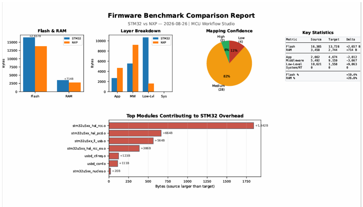
Figure 4.12: Generated footprint report showing the global and per-layer comparison outputs.
