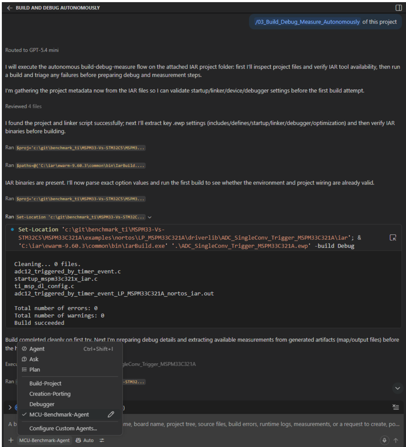
Figure 5.4: Benchmark campaign initiated through the custom agent in VS Code Copilot Chat.
