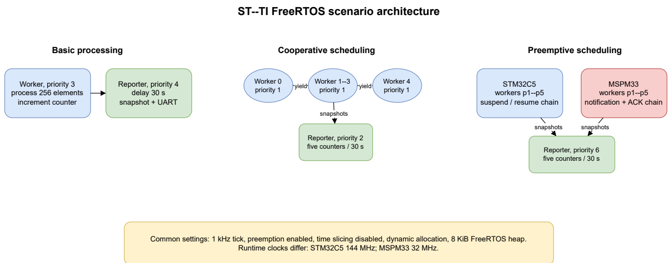
Figure 7.3: Task architecture of the three ST-TI FreeRTOS scenarios. The preemptive scenario deliberately shows the non-equivalent synchronisation paths found in the measured projects.
