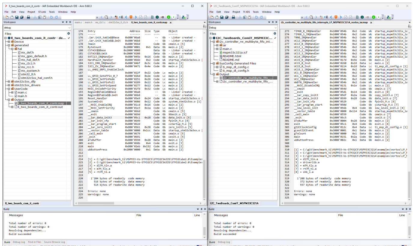
Figure 7.2: Matched functional scenario builds and linker-map memory totals in IAR EWARM.
