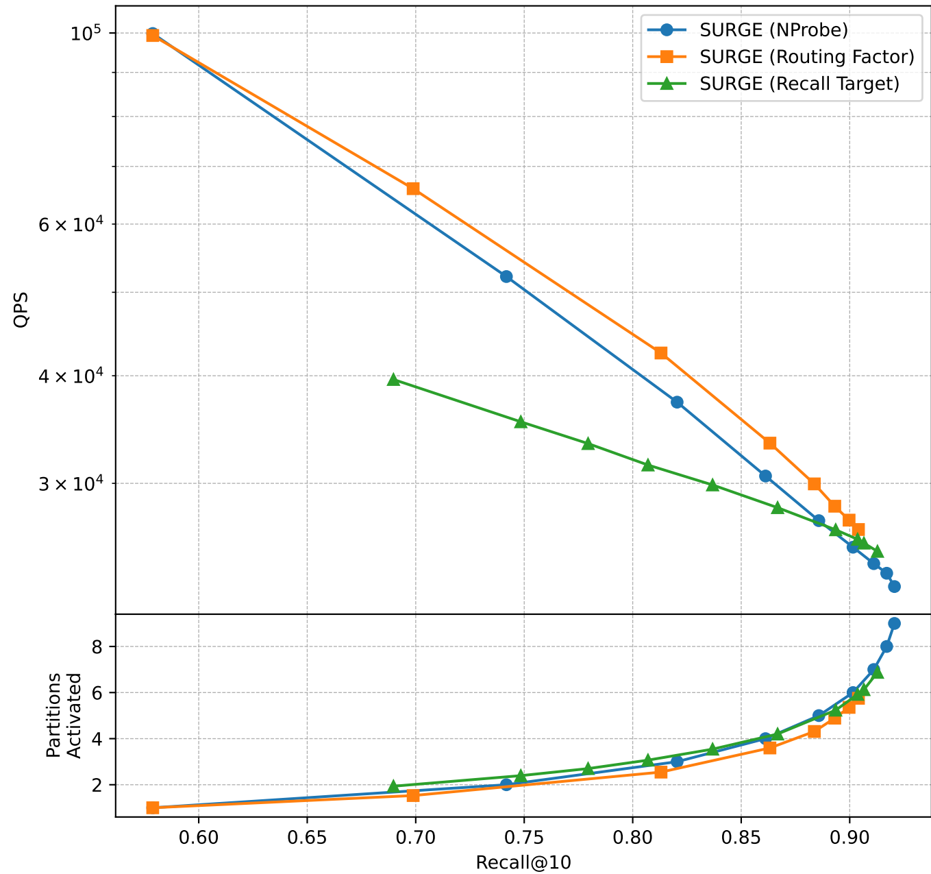
MSTuring500M, 10 partitions
