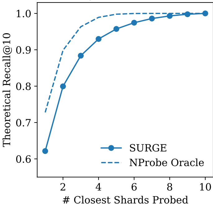
MSTuring-500M, 10 partitions
