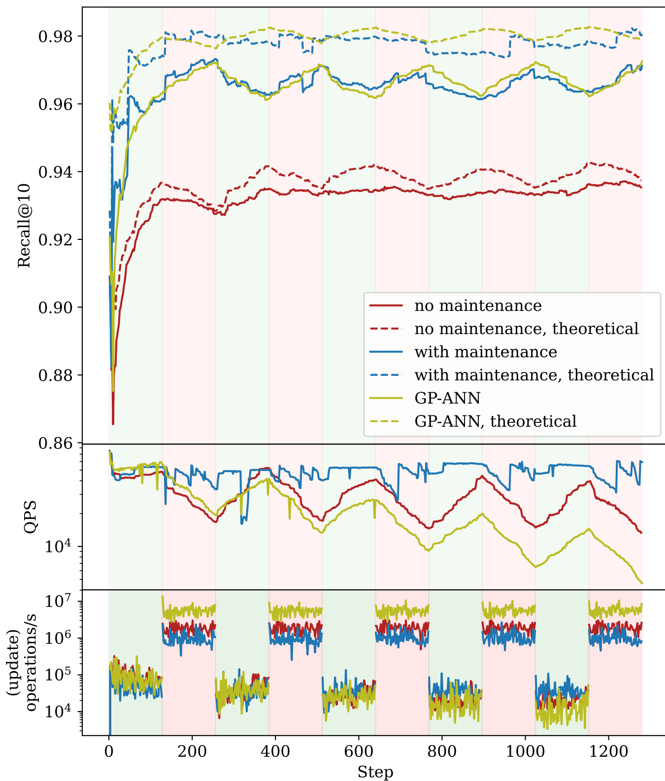
SIFT-100M-clustered
