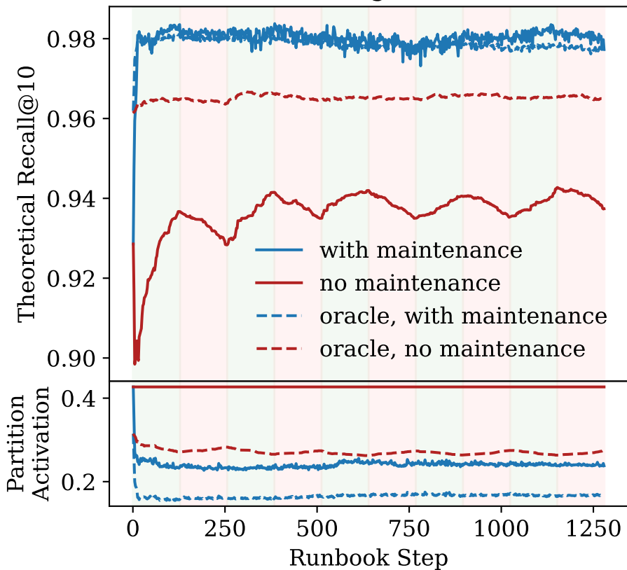
SIFT-100M-Clustered, 10 partitions RecallTarget = 0.9
