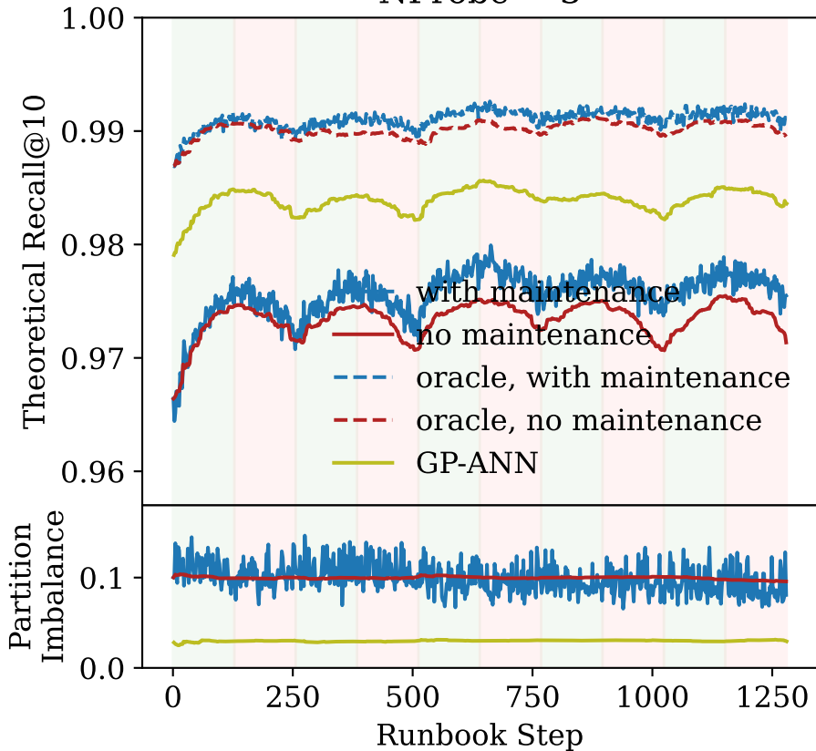
SIFT-100M-Uniform, 10 partitions NProbe = 3
