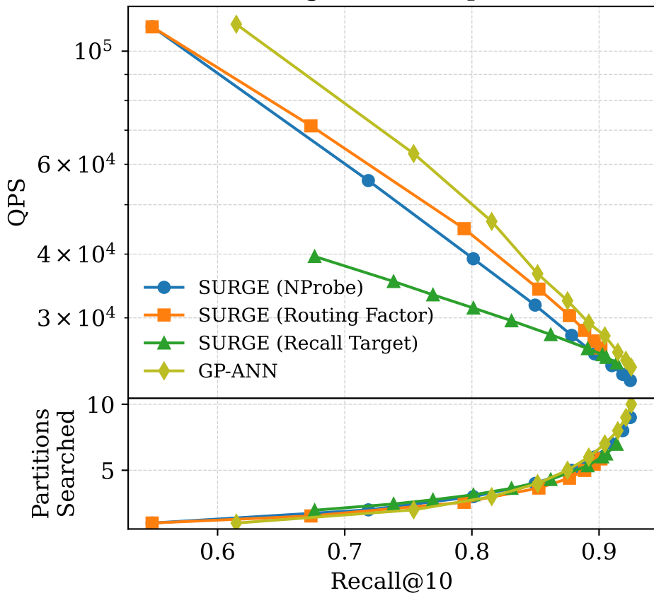
MSTuring-100M, 10 partitions
