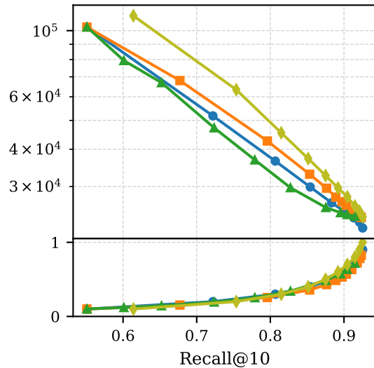
MSTuring-100M
