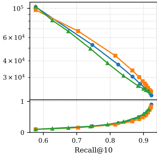
MSTuring-500M
