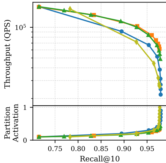
SIFT-100M
