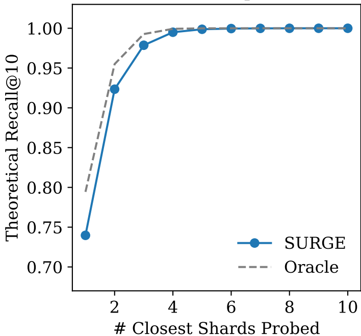
SIFT-500M, 10 partitions
