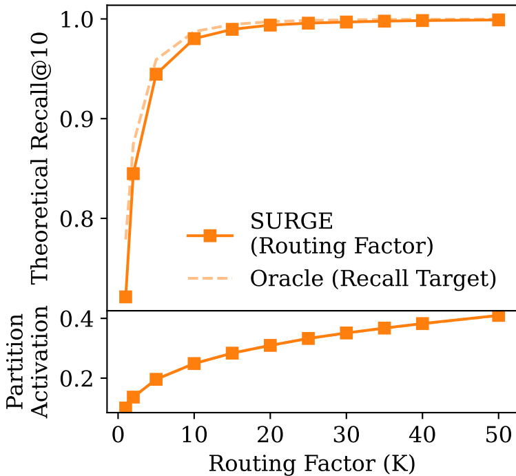
SIFT-100M, 10 partitions
