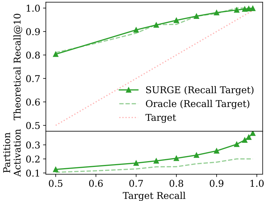
SIFT-500M, 10 partitions
