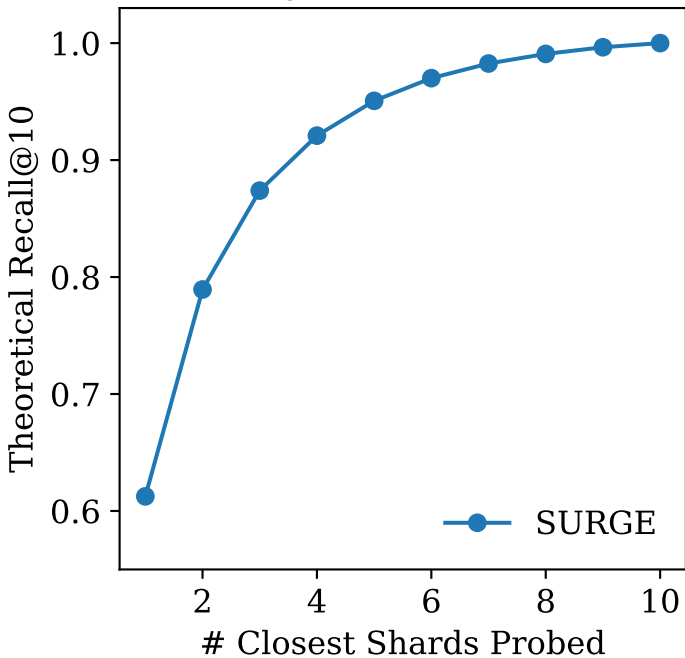
MSTuring-500M, 10 partitions
