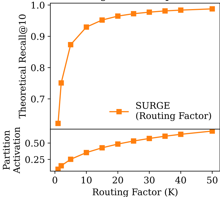
MSTuring-500M, 10 partitions
