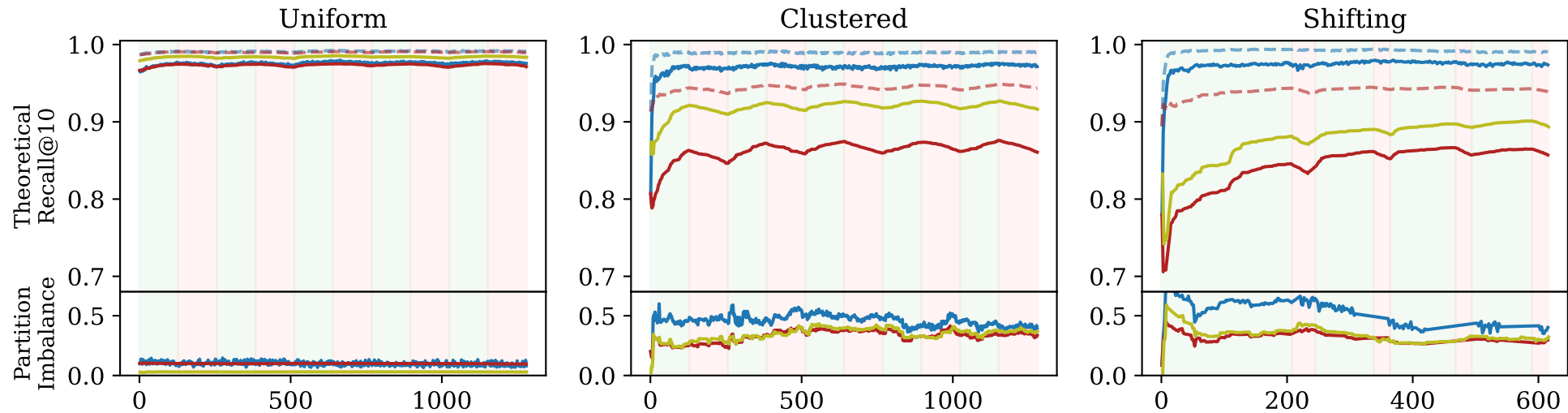
SIFT-100M (NProbe = 3)
