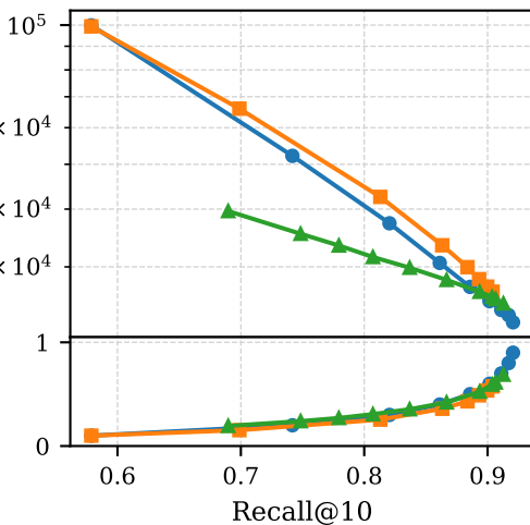
MSTuring-500M
