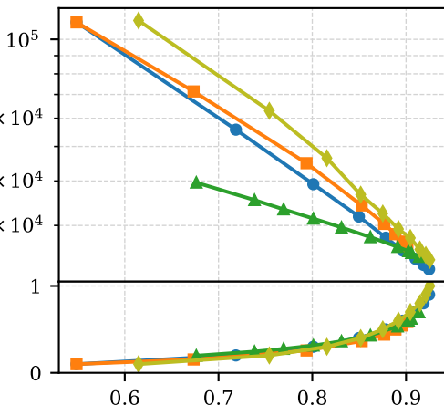
MSTuring-500M
