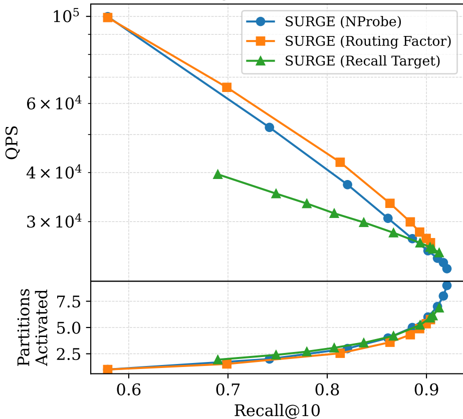
MSTuring500M, 10 partitions
