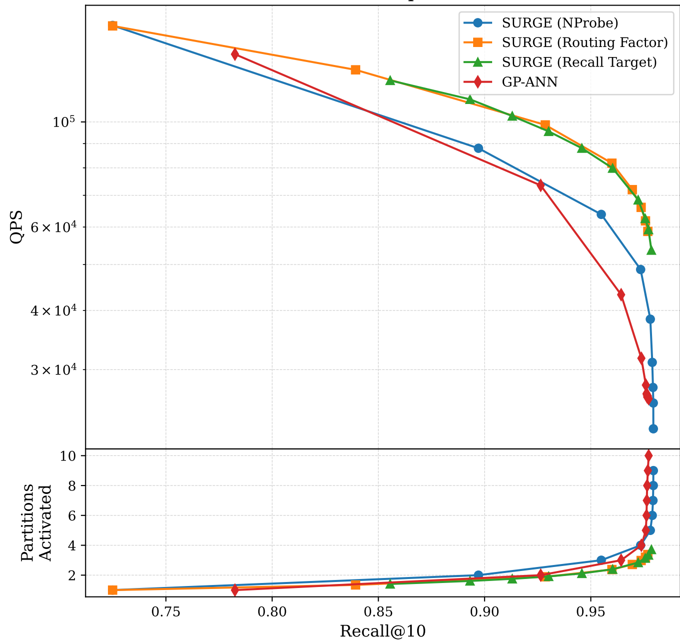
SIFT100M, 10 partitions
