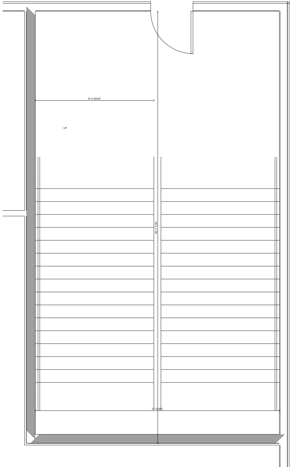
1 ENLARGED STAIR PLAN SCALE: 1/2" = 1'-0"
