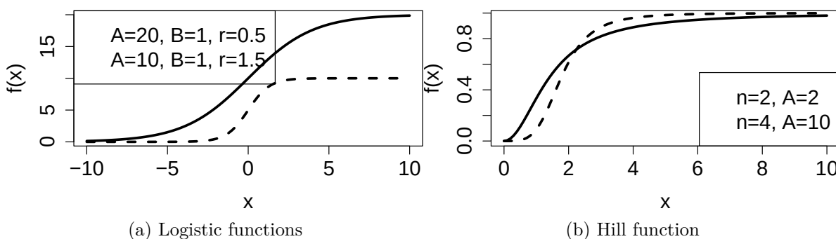
Figure 2.2: Examples of functions with sigmoidal-shaped graphs
