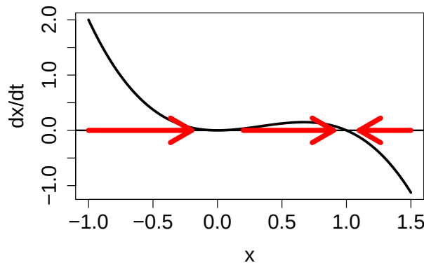
Figure 7.5: a) plot of the defining function of the ODE dx/dt = -x^3 + x^2 with direction of flow of x(t) indicated with arrows on the x-axis; b) plot of solutions x(t) of the ODE starting with three initial values
