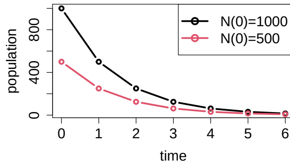
Figure 5.3: Plots of solutions of linear difference equations: a) N(t+1) = 2N(t) with different initial values; b) N(t+1) = 0.5N(t) with different initial values
