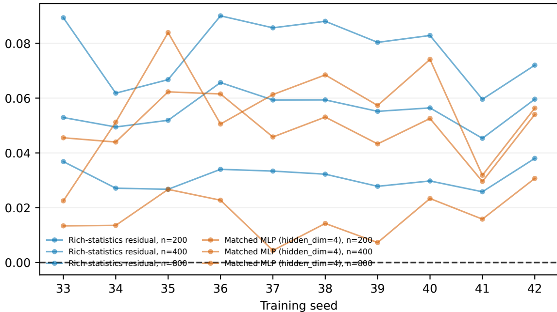
Paired external Pearson delta
