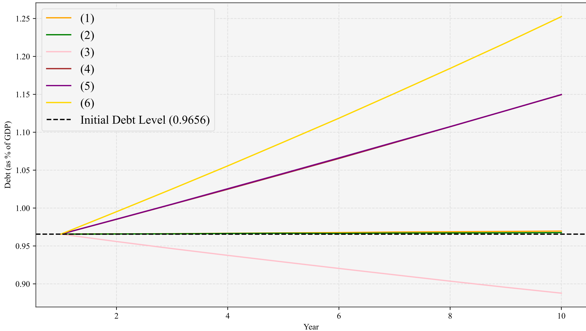
Mean Debt-to-GDP Ratio
