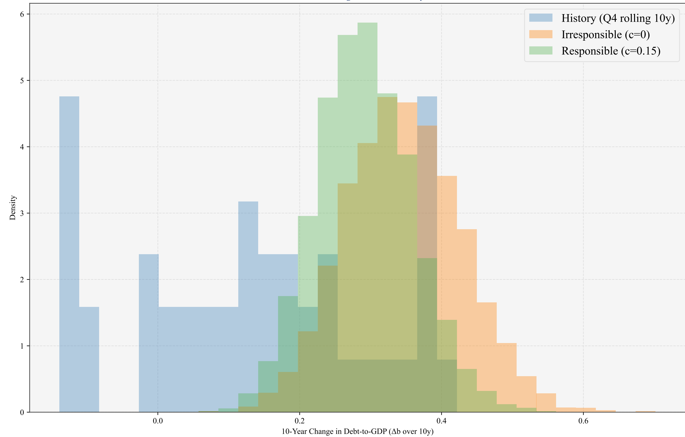
Distribution of 10-Year Change in Debt: History vs. Simulations
