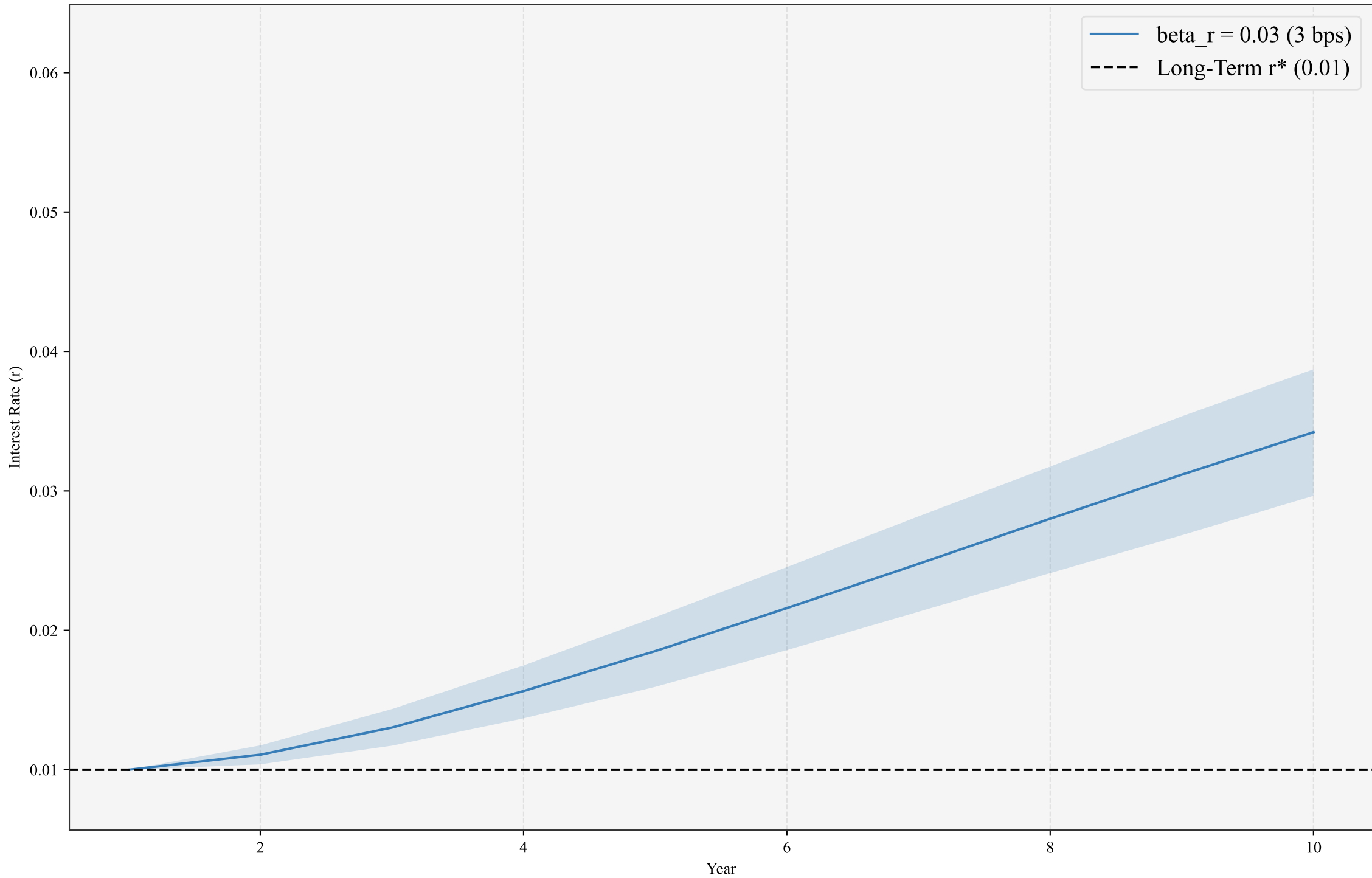
Median and Percentiles of Interest Rate (r) - Irresponsible Fiscal Regime
