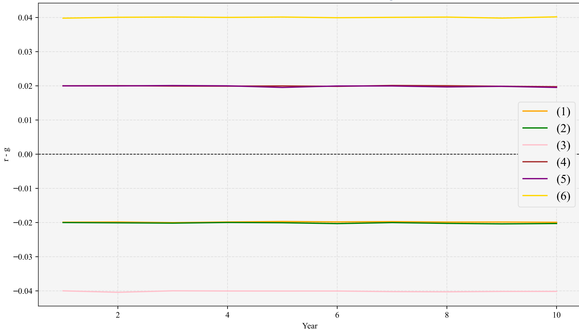
Mean Interest-Growth Differential ( r - g )
