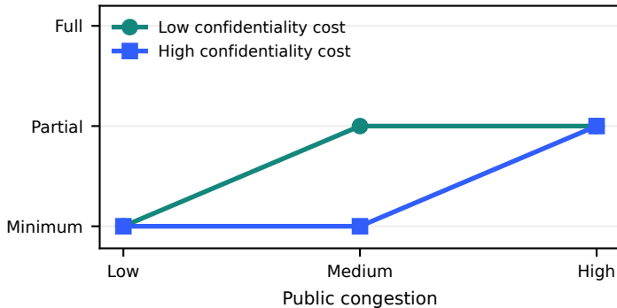
A. Unique pure BNE by type
