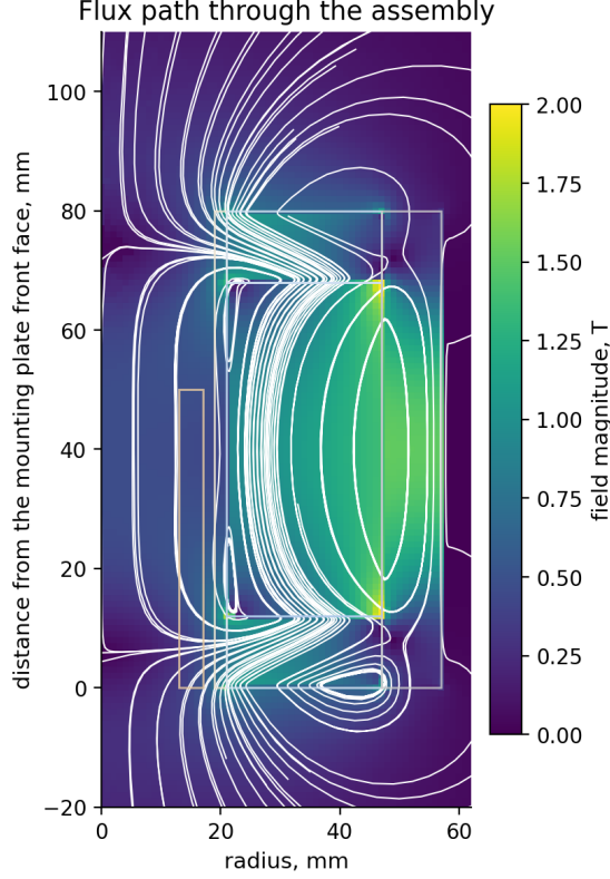
Nearest exported build: 12 mm end caps, 94 mm magnet OD. The flux path is the same for 16 mm caps.
