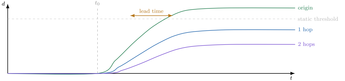
Figure 4.1: The silent regime of (4.1)–(4.4). The origin crosses a static threshold late; the joint pattern across hops is distinctive early. That gap is what the graph buys.
