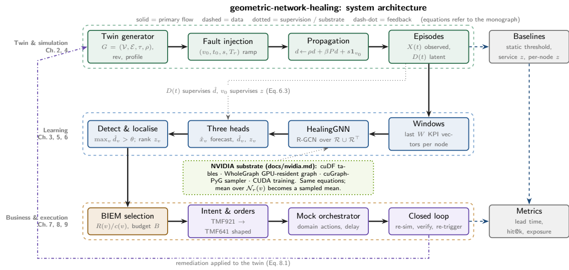
Figure A.1: System architecture of the repository. Equation numbers refer to this document.
