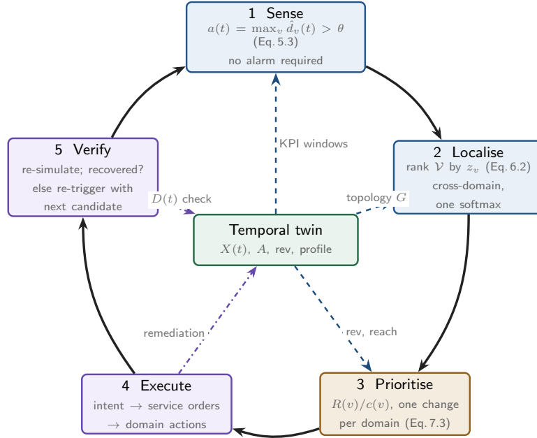
Figure 8.1: Five stages around a twin. The only input is the KPI stream; the only output is an ordered set of per-domain actions. Stages 1–2 are the learned model, stage 3 a one-line rule, stages 4–5 plumbing and verification.
