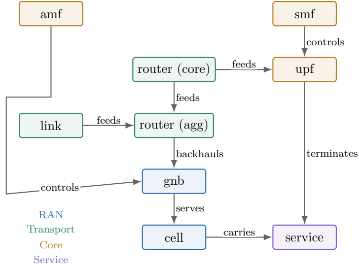
Figure 2.1: The node types and relations of (2.1), colour-coded by domain. Arrows point in the direction a fault propagates. A service is the trigger surface: a service-layer symptom is the only input the healing loop needs.
