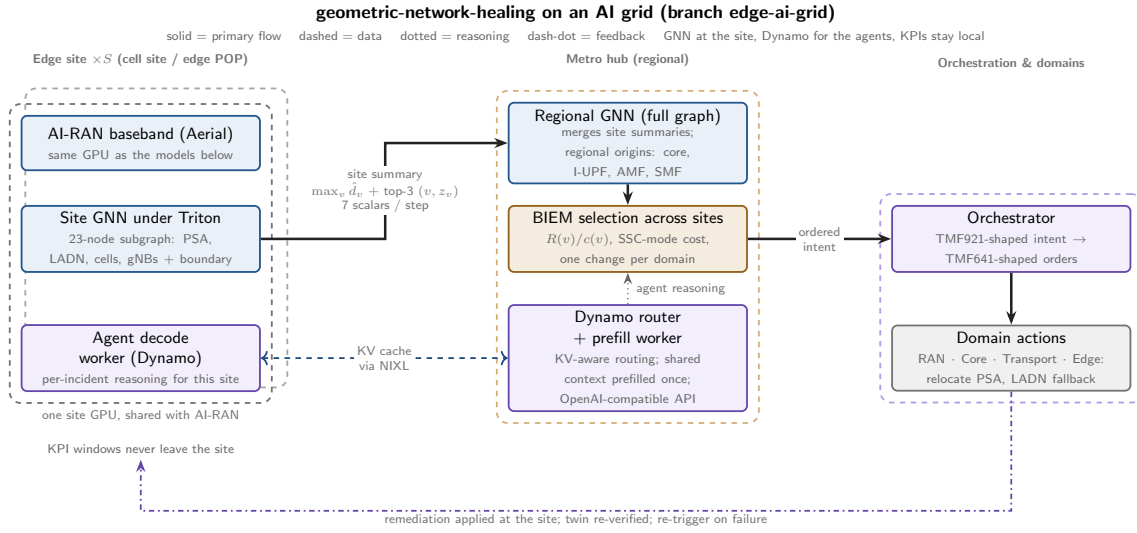
Figure 12.2: Deployment shape on an AI grid. The site GNN and the agent decode worker share the site GPU with the AI-RAN baseband; the hub holds the regional full-graph pass, the business layer, and Dynamo’s router and prefill worker. Only site summaries go up; only remediation comes down.
