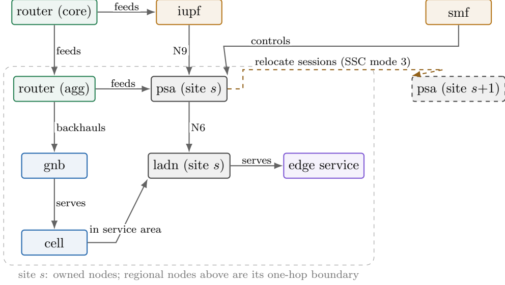
Figure 12.1: One edge site in the extended twin (12.1). The PSA and LADN are owned by the site; the core router, I-UPF and SMF are regional and appear in the site’s subgraph only as boundary context. The dashed relocation is a remediation action, not a propagation edge.
