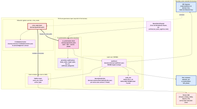
Figure 2: Governance layer zoom. The TMF688 audit event carries the proposal, the guardrail result, the sandbox verdict, the optional companion intent with its dispatch result, and the seven-field ReversibilityProfile. The co-authorization contract sits between draft and commit. The Killswitch (crisis_mode) is the global override.
