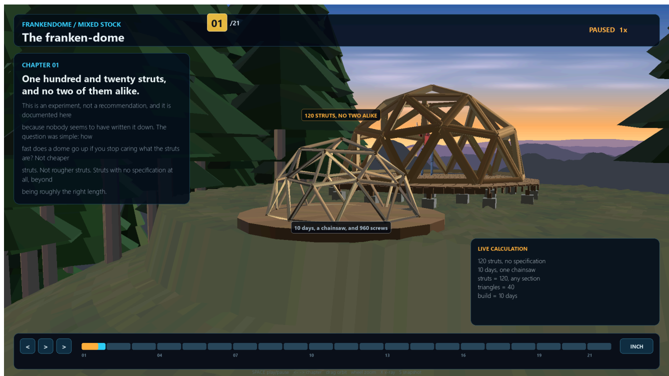
The frankendome: it stood, and no two members matched.
