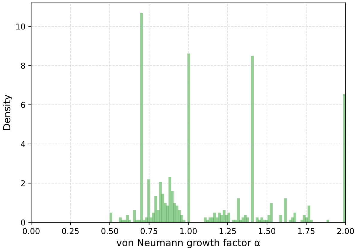
Distribution of \alpha
