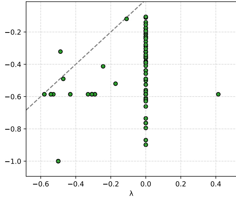
\mu < 0
