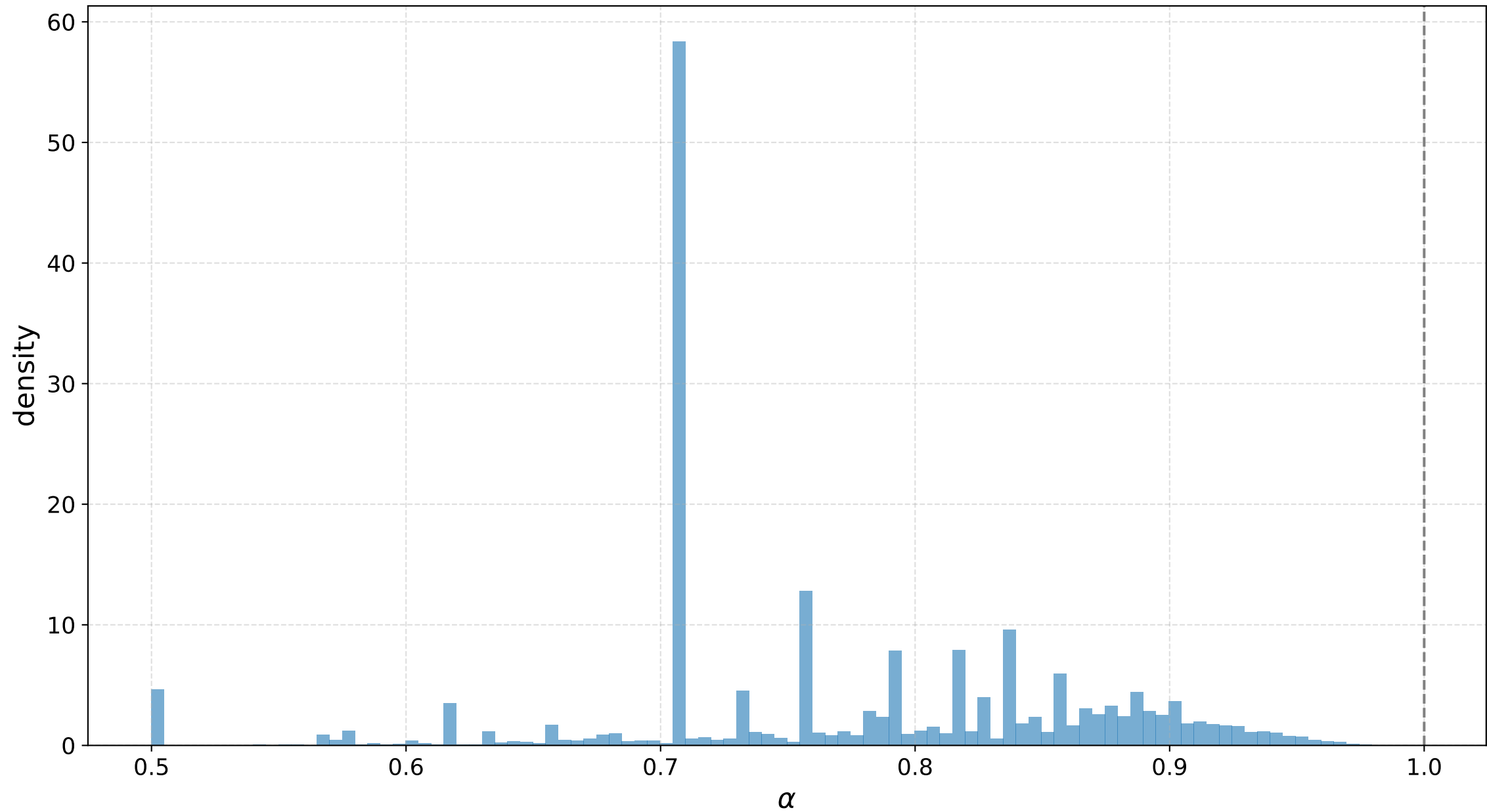
Distribution of \alpha ( \alpha < 1 )
