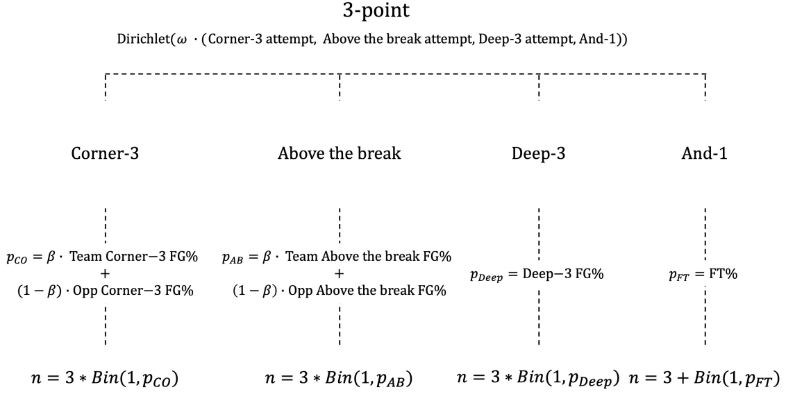
Figure S3: 3-point attempt (3PA) sub-model (Base Model).
