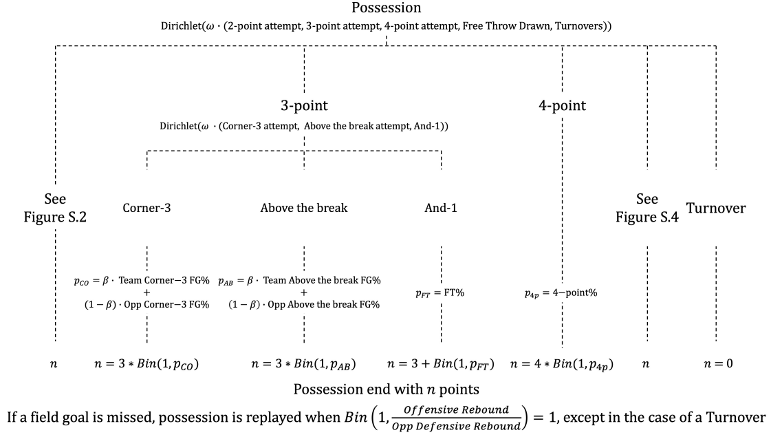
Figure S5: Alternative possession model incorporating a 4-point attempt (4PA).
