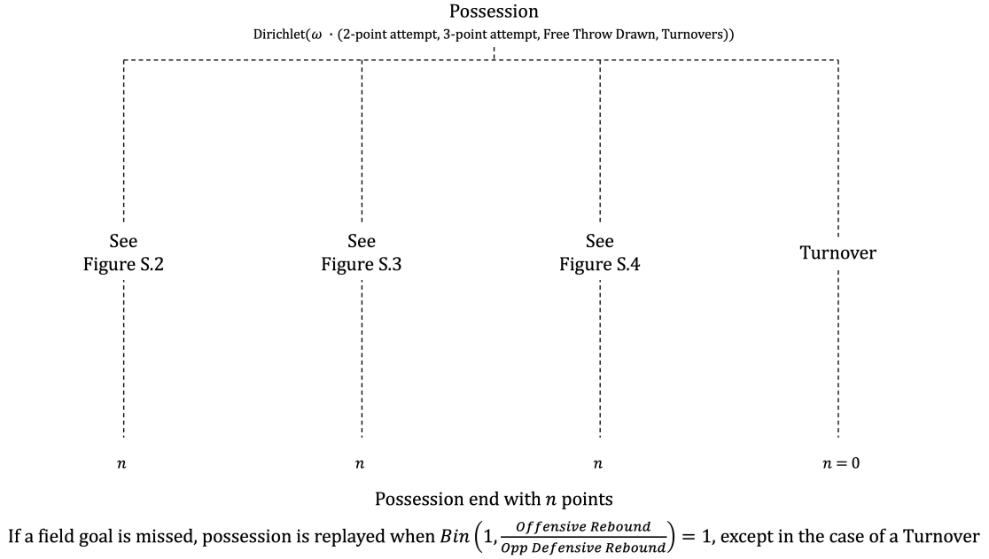
Figure S1: Top-level possession model (Base Model).
