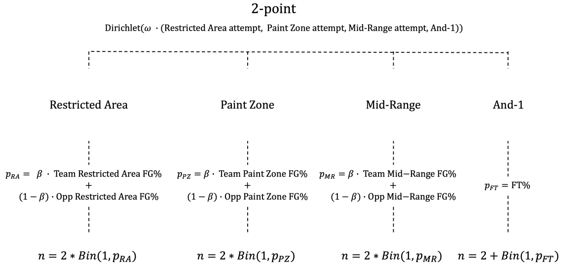
Figure S2: 2-point attempt (2PA) sub-model.
