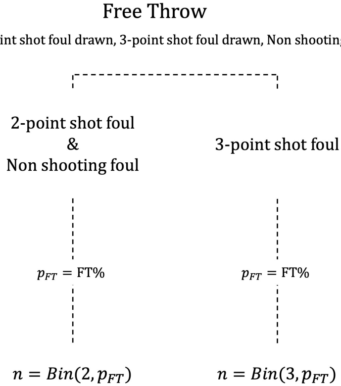
Figure S4: Free Throw Drawn (FTD) sub-model.
