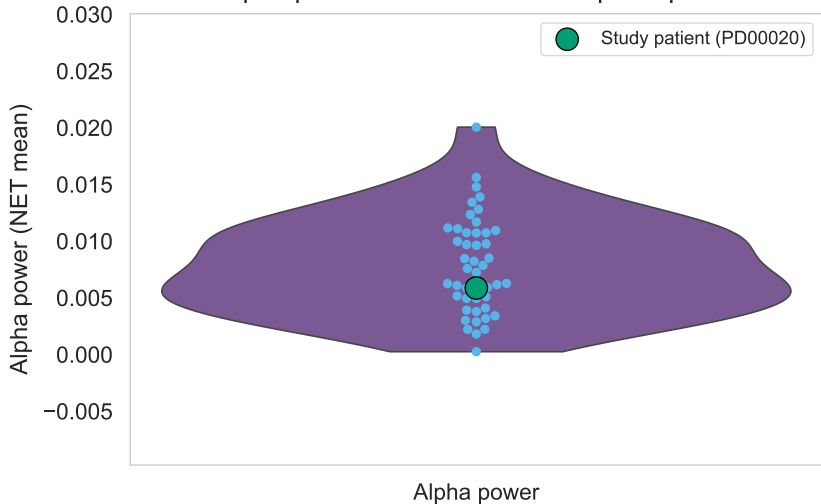
Alpha power distribution across participants
