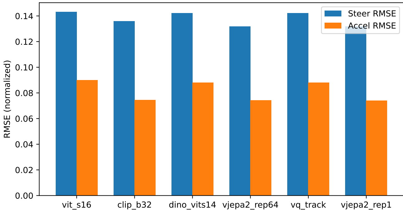
P0 RMSE by Encoder
