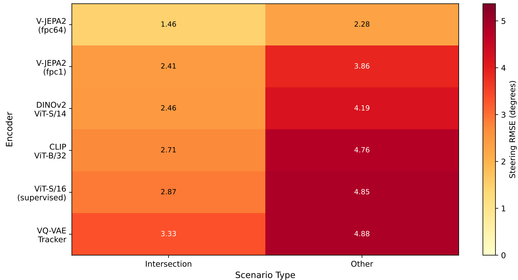
Per-Scenario Steering RMSE by Encoder
