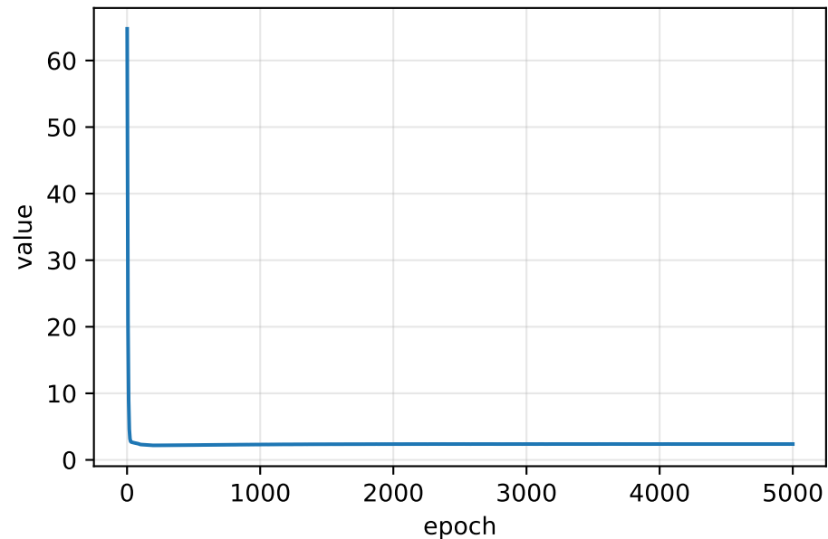
Beta
