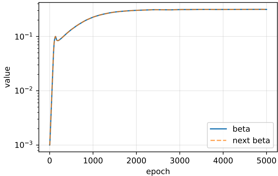
Beta
