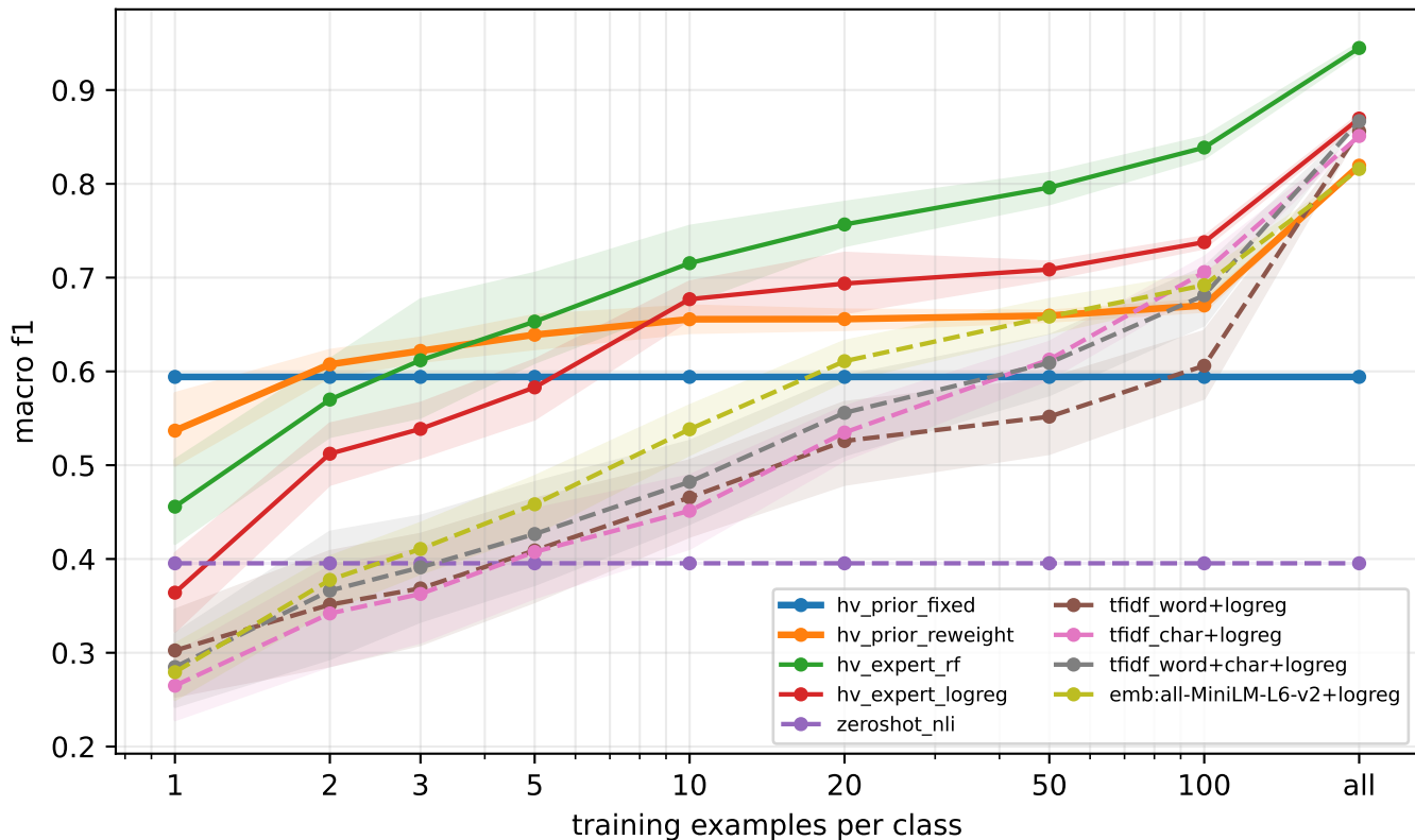
TREC-6 low-label learning curve (finecat-nli-l)
