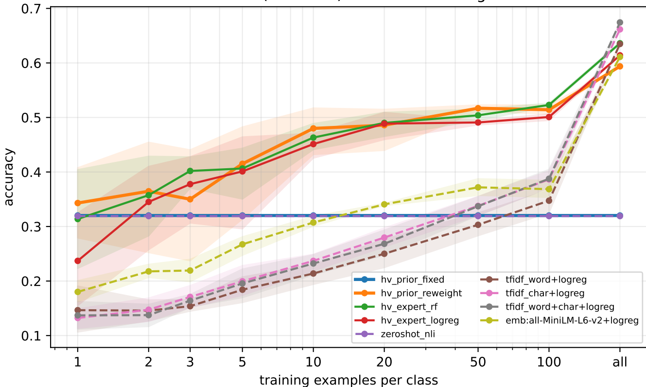
GoEmotions (Ekman-7) low-label learning curve
