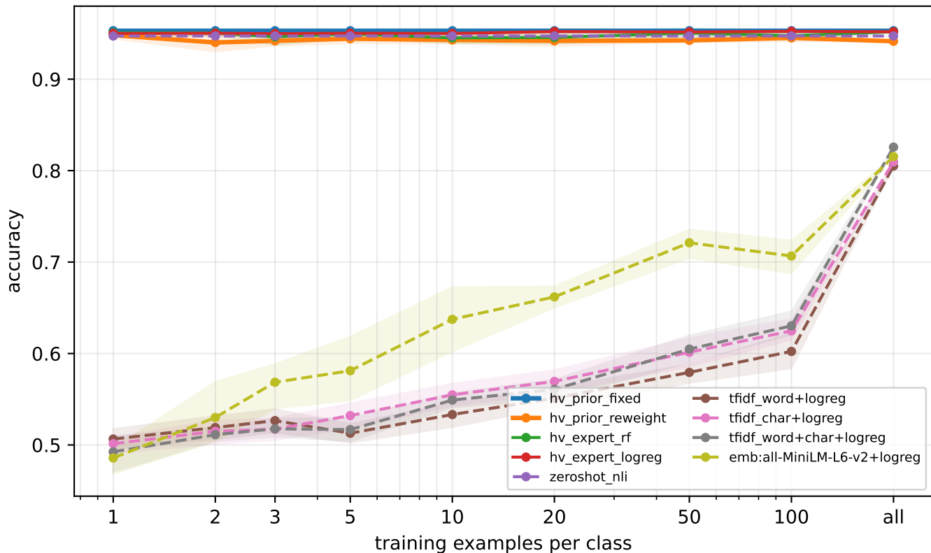
SST-2 low-label learning curve (finecat-nli-l)
